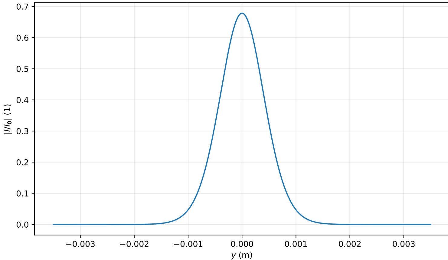
Intensity profile I(x=0, y, z=1.911)/I_0 , P_{in}=0.3P_{cr} , artificial time
